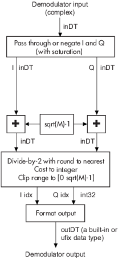
Signal-Flow Diagrams with Trivial Phase Offset and Denormalization Factor Equal to 1
